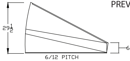
6/12 PITCH
